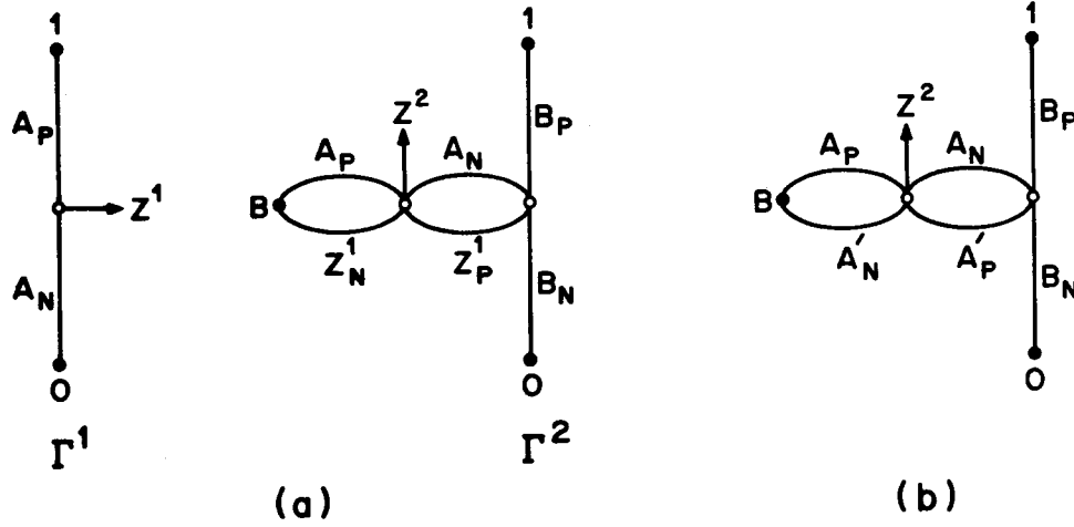
Figure 4.2 (a) XOR implementation using transmission gates; (b) \tilde{\Gamma}^2 .
