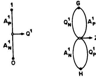
Figure 6.3 C-graph \Gamma^3 .
