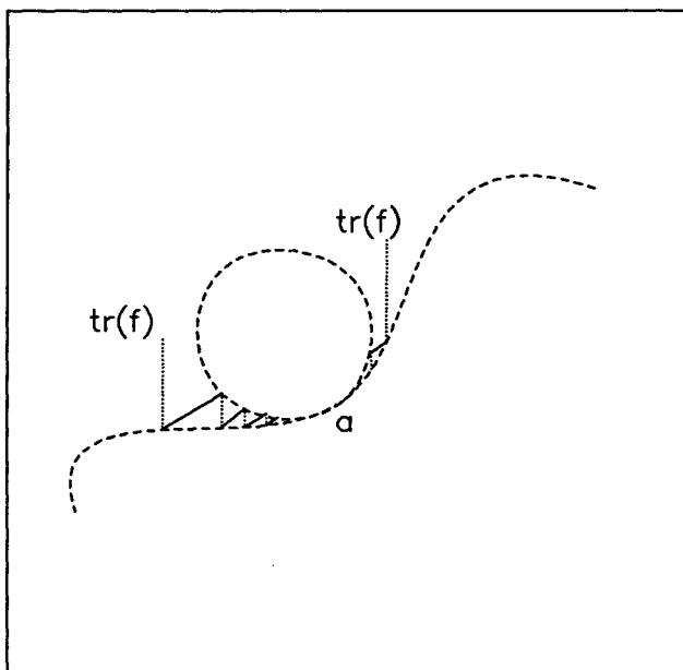
Figure 5: tr(f) is twice geometrically differentiable at a but not zero times geometrically continuous in any neighborhood of a
