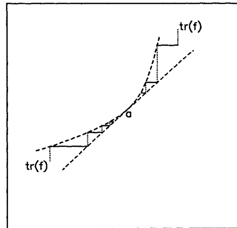
Figure 4: \text{tr}(f) is once geometrically differentiable at a but not zero times geometrically continuous in any neighborhood of a
