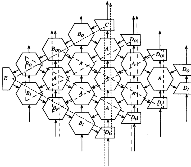
Fig. 7-2: Paths taken by three matrix elements.
