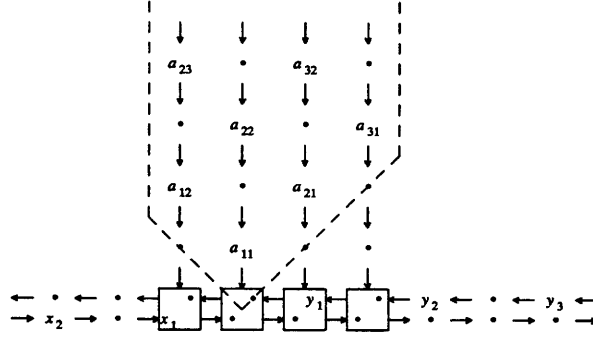
Fig. 2-4: Systolic system for computing the band matrix-vector multiplication in Fig. 2-3.
